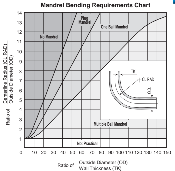
Fig. R59 — Mandrel bending requirements chart
