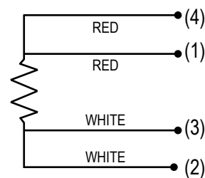
4-Wire
