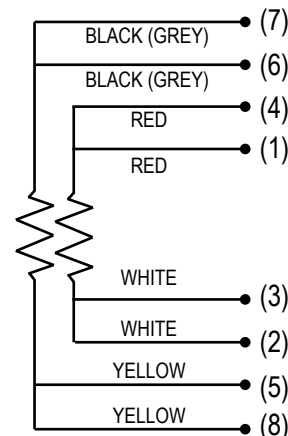
Dual 4-Wire
