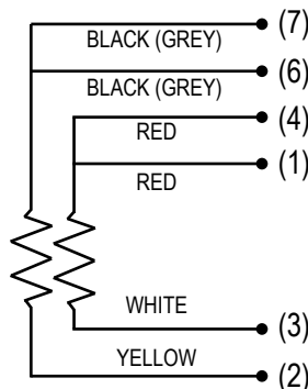
Dual 3-Wire
