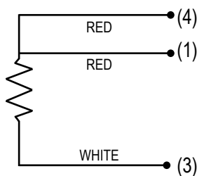
3-Wire
